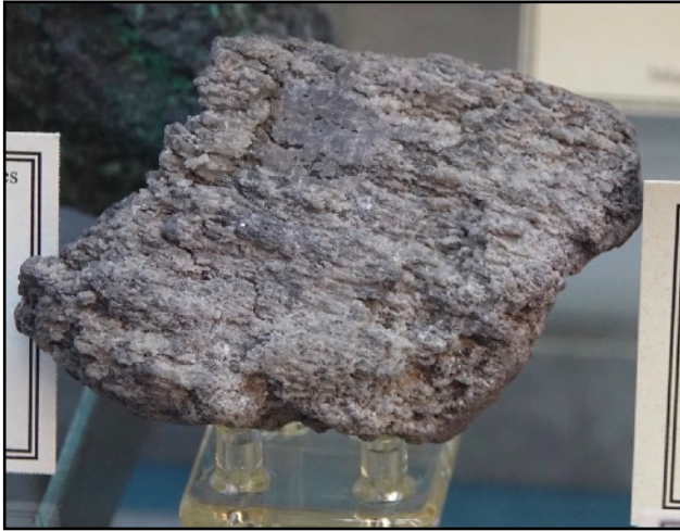
Chlorargyrite (AgCl) - Caroline Mine, Lake Valley Mining District, Sierra County
