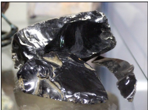
Obsidian - Probably not mined in the Black Range but used by the Mimbres people. Specimen at Mimbres Cultural Heritage Site, San Lorenzo, NM
