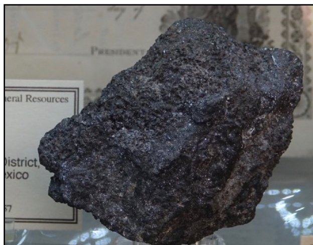
Pyrargyrite ( \text{Ag}_3\text{SbS}_3 ) - From the Pelican Mine, Hermosa Mining District, Sierra County
