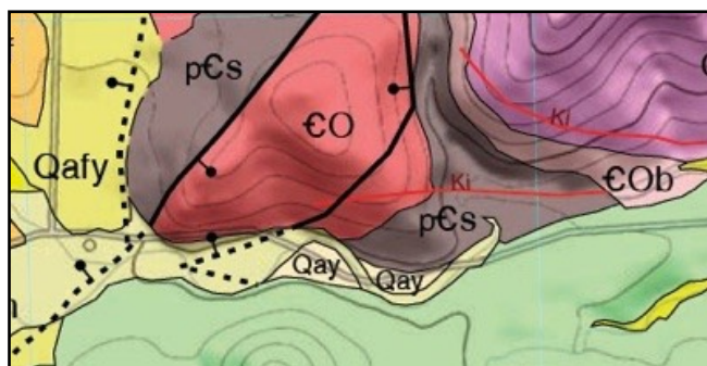
PALEOZOIC BEDROCK
